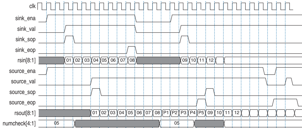
Figure 3-3. Variable Encoding
